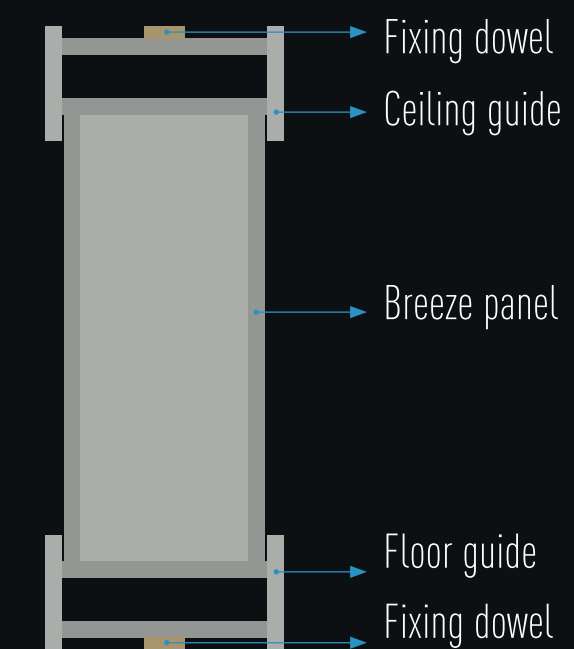
Mounted guide - side view
