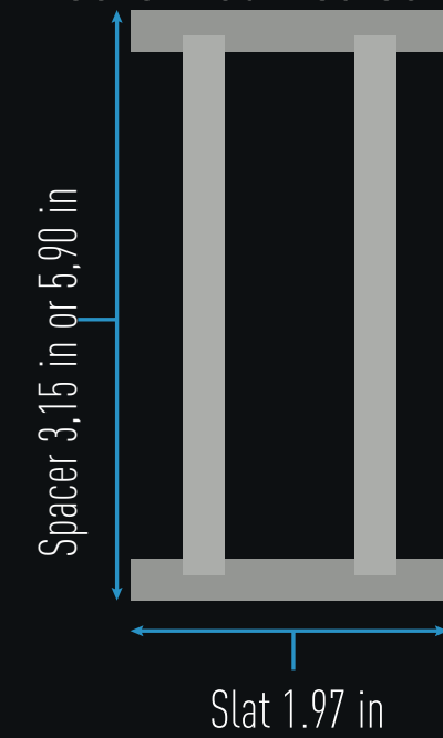
Breeze mounted column - top view
